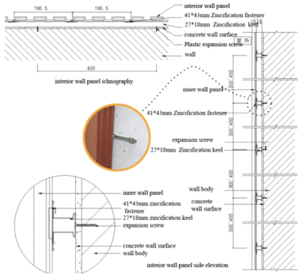
Zncification Clips(Side)
